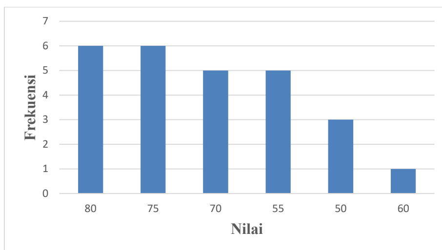
Gambar 1 Diagram Batang Nilai Pre-Test Kelas IV
