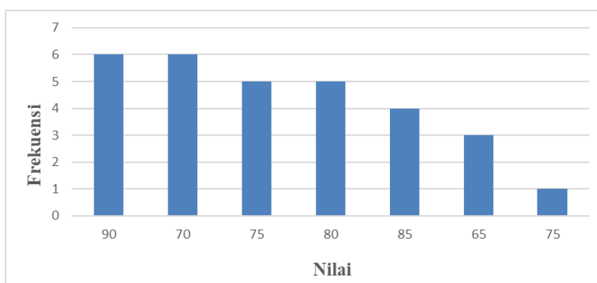
Gambar 2 Diagram Batang Nilai Post-Test Kelas IV
